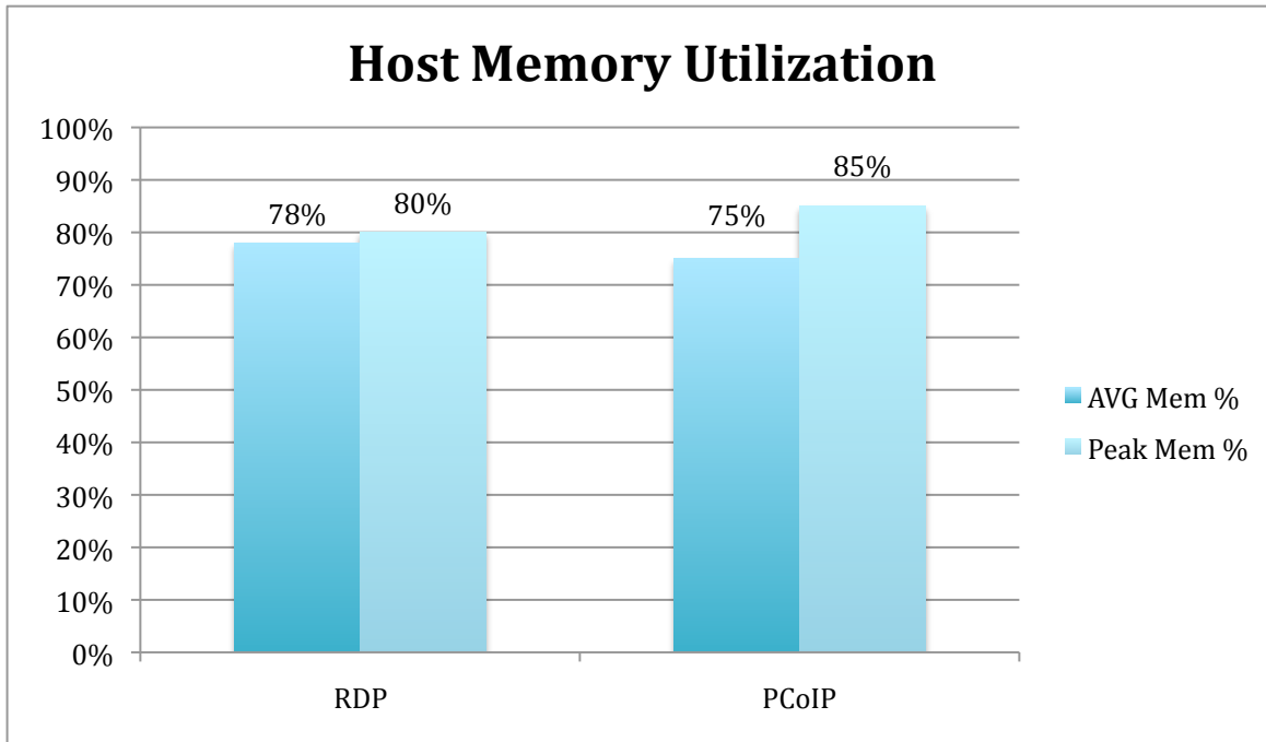
Figure 11 – Task Worker – Protocol Memory Comparison
