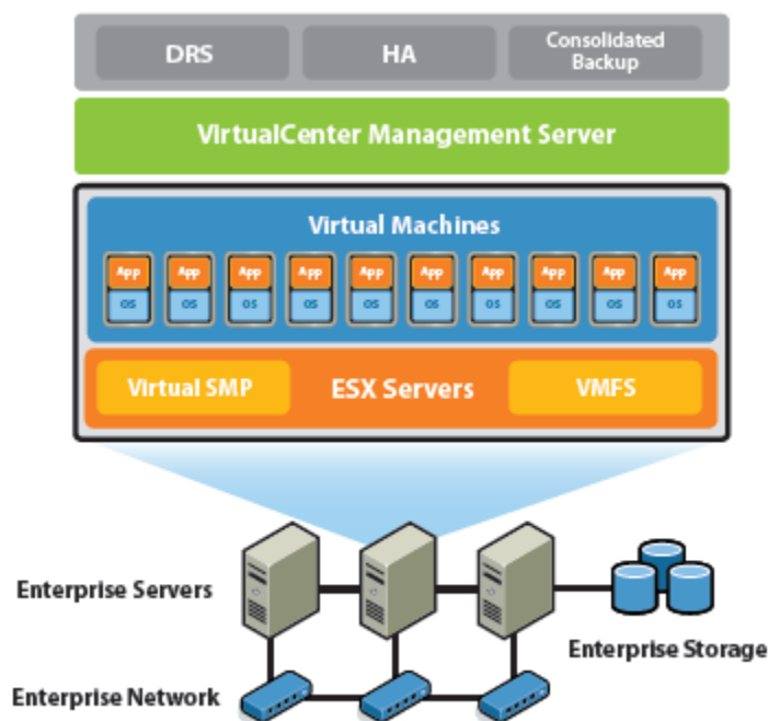
Figure 1: VMware Infrastructure
