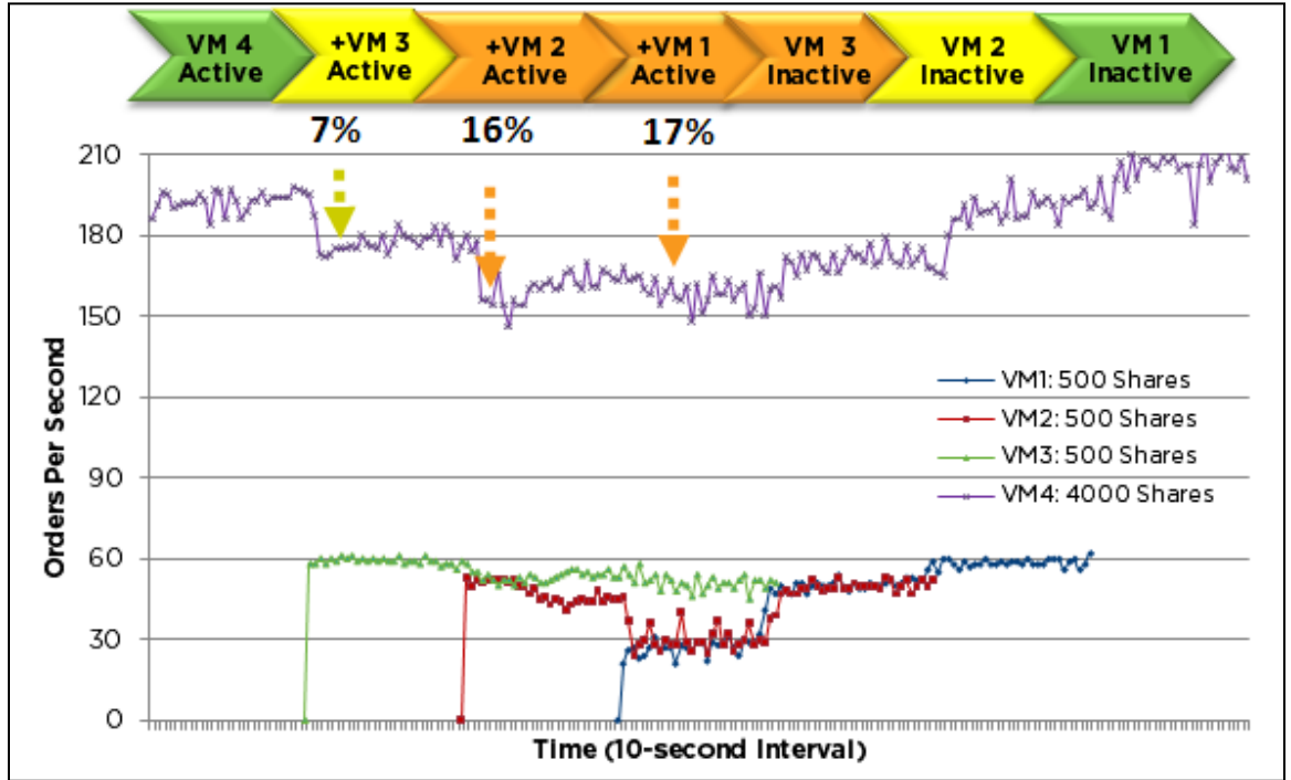
Figure 13. Test Results when SIOC Was Turned On
