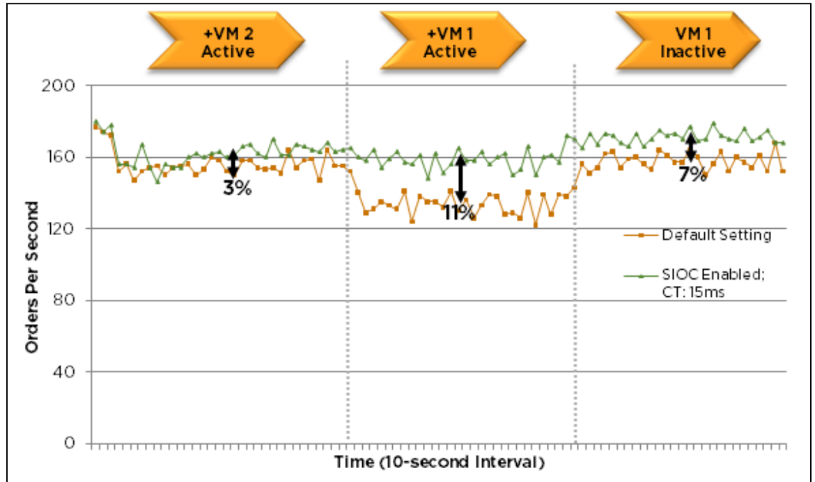
Figure 14. DS2 Throughput of the High Priority Workload with and without SIOC Enabled
