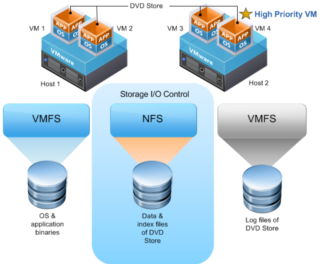
Figure 1. Test Bed Layout with 4-VM Configuration
