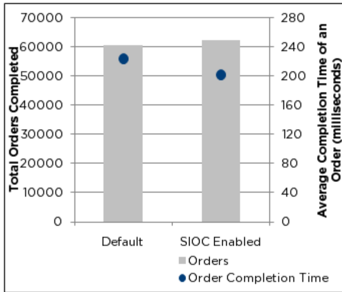
Figure 2. Impact of Storage I/O Control on Performance of DVD Store Workload in VM 4
