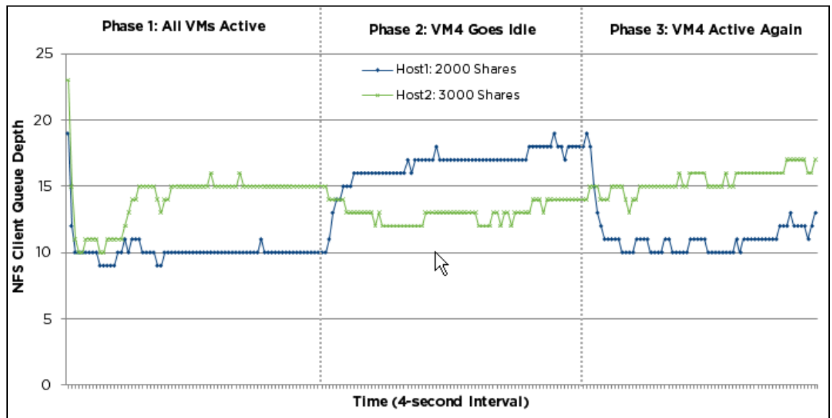
Figure 11. NFS Client Queue Depth in Each Host
