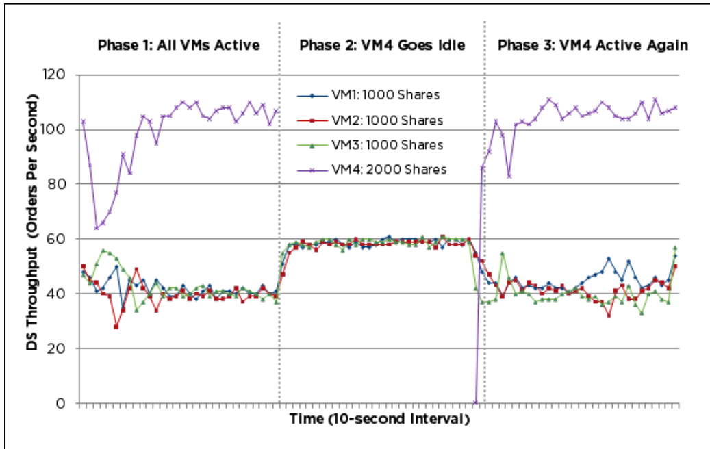
Figure 7. Application Throughput of all VMs in Different Phases
