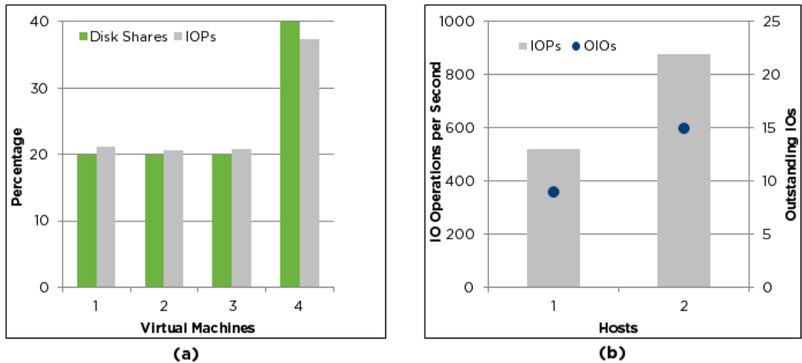
Figure 4. I/O Performance of the VMs when SIOC Was Enabled
