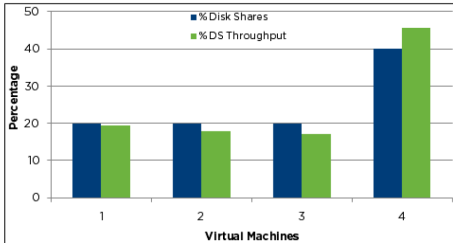
Figure 10. Ratios of DVD Store Throughput and VM Disk Shares in Phase 3
