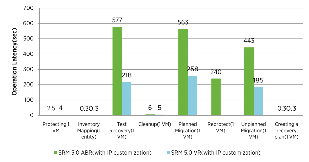
Figure 2. Major SRM 5.0 operations - latency overview
