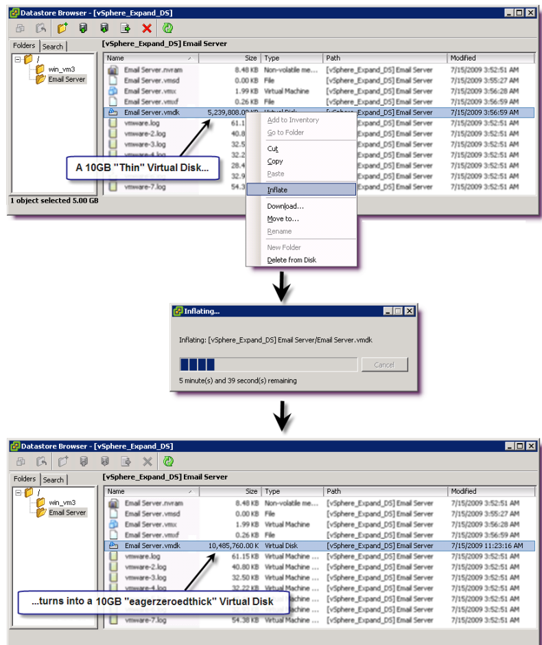
Figure 25. Inflating a thin virtual disk to the eagerzeroed thick format
