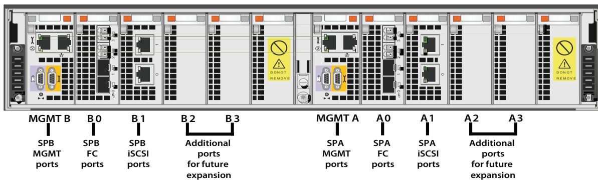
Figure 1: EMC CLARiiON CX4-240 ports
