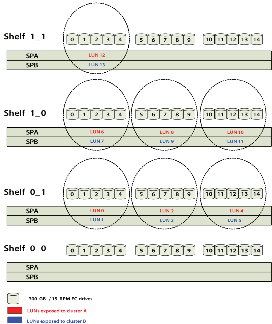
Figure 4: EMC CX4-240 RAID group configuration
