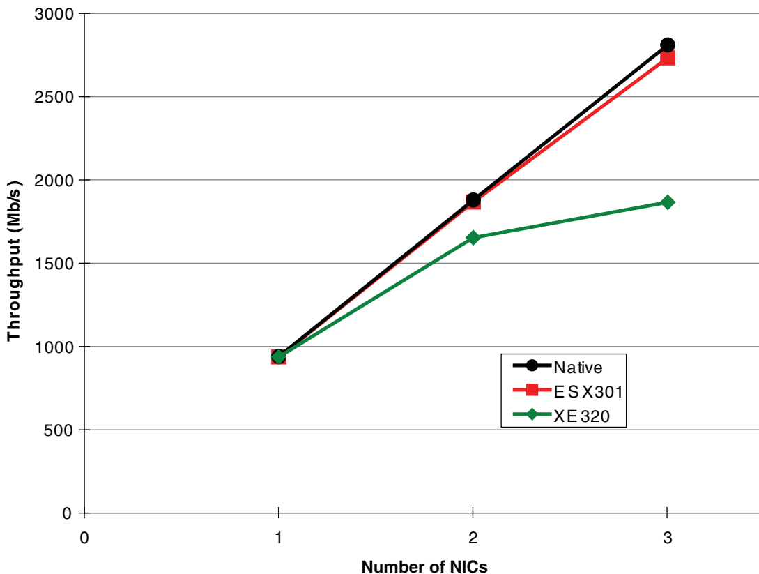
Figure 2. Netperf Receive Results
