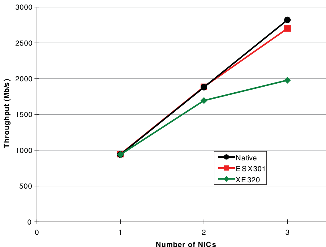
Figure 1. Netperf Send Results
