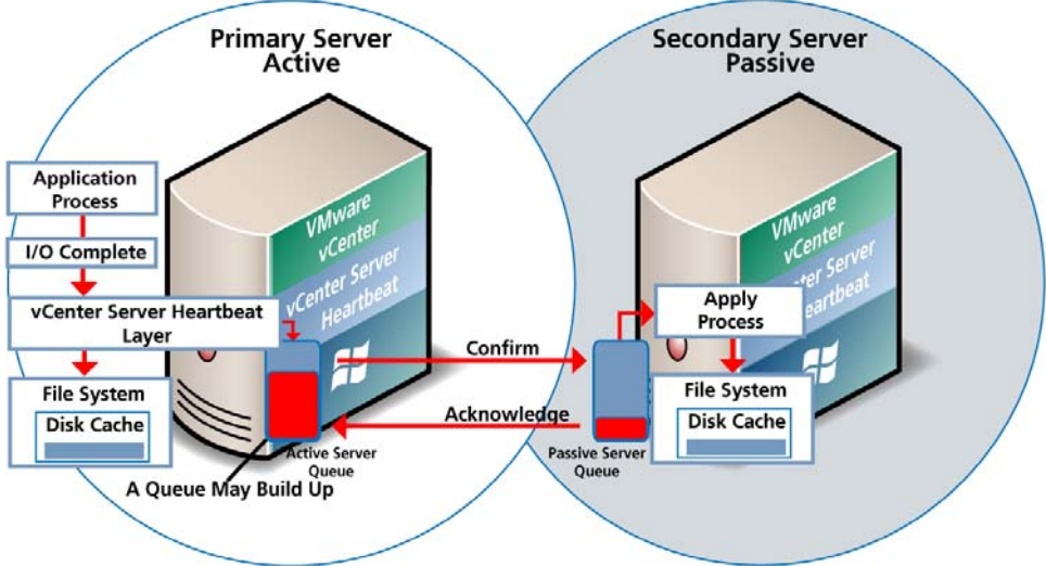
Figure 1-3. Apply Process
