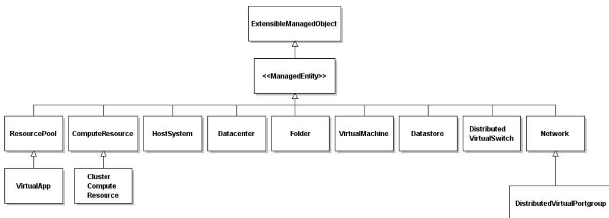
Figure 2-1. ExtensibleManagedEntity Hierarchy
