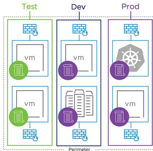
FIGURE 3: Network Segmentation
