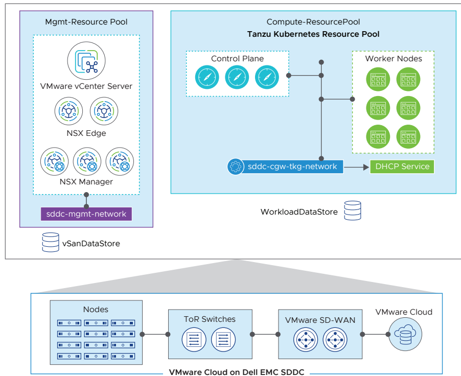
Figure 2: Tanzu Kubernetes with VMware Cloud on Dell EMC
