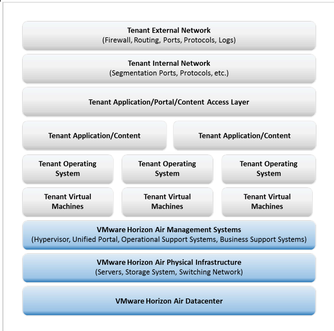
Figure 1. The "Responsibility Stack", illustrates the limits of control and areas of individual responsibility for VMware and tenants of its Horizon Air
