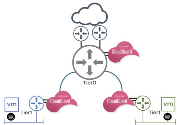
Figure 1: Check Point CloudGuard with North-South service insertion for NSX-T Data Center protects against advanced threats at the edge.
