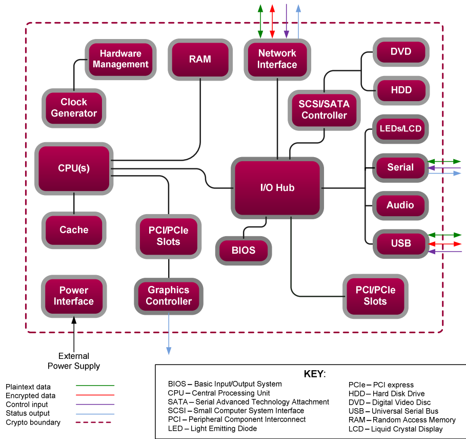
Figure 2 – HP ProLiant Server Block Diagram
