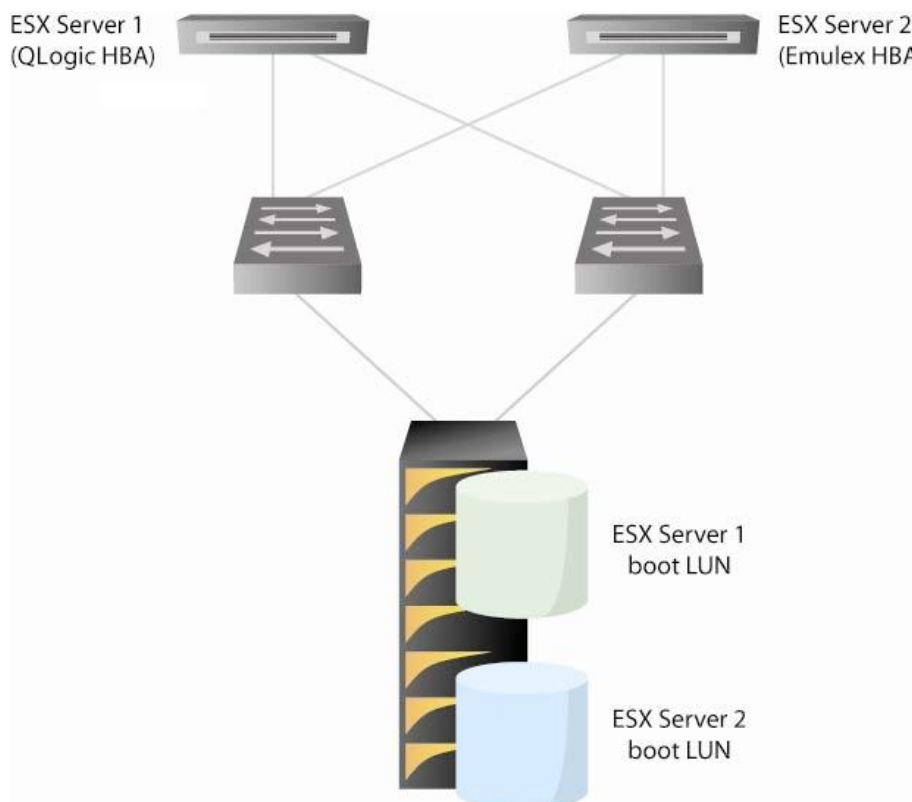
Figure 7. A "Boot from SAN" configuration
