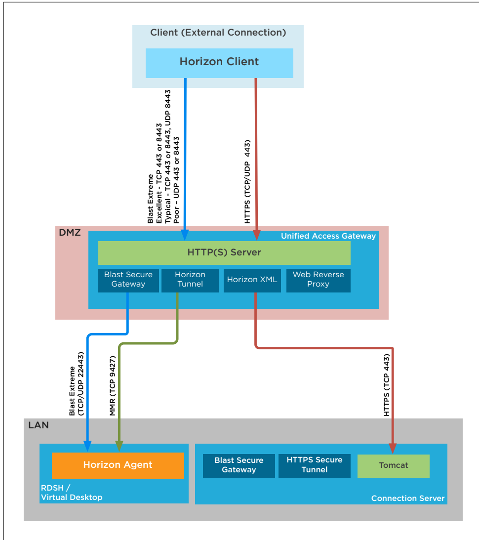
Figure 3: External Connection from Client to Agent Through the Unified Access Gateway
