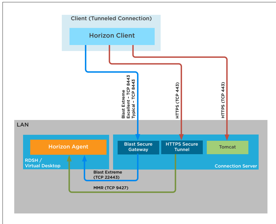
Figure 2: Tunneled Connection from Client to Agent Through the Connection Server
