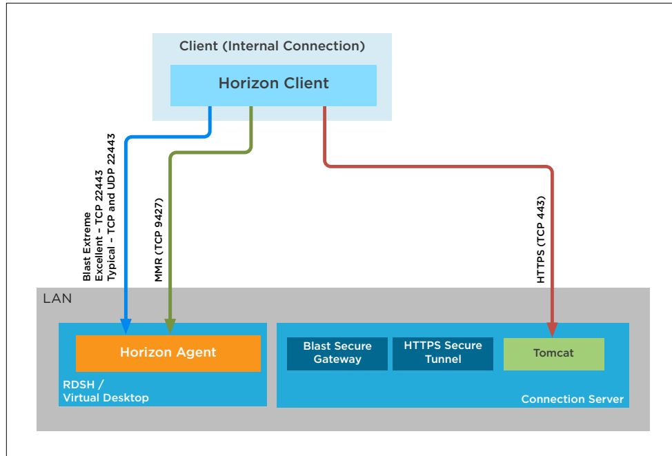
Figure 1: Internal Connection from Client to Agent Using Blast Extreme
