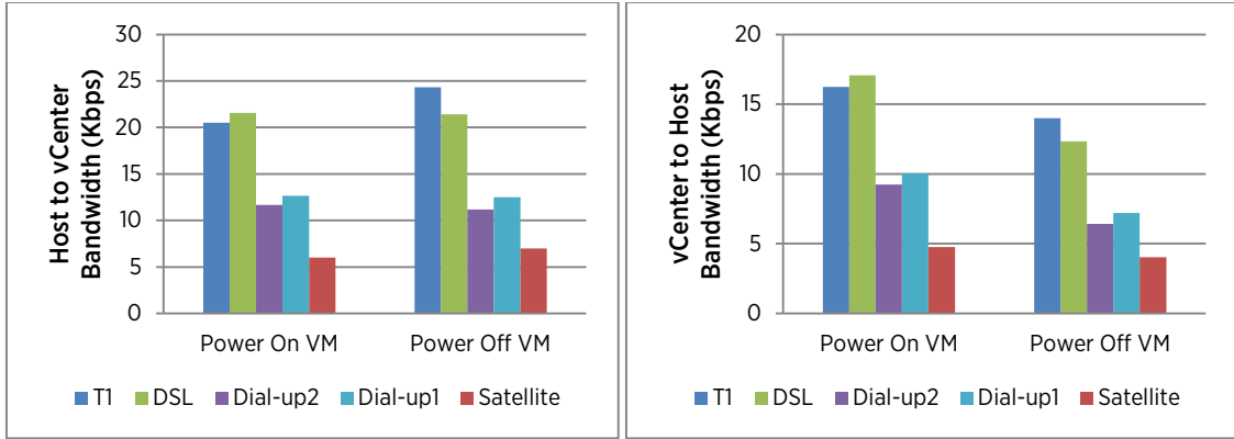
Figure 8. Bandwidth consumption for powering on and off a VM. The more bandwidth a network pipe has, the more bandwidth is used for a vCenter task. However, the network pipes are not saturated for all the five representative low-bandwidth cases.
