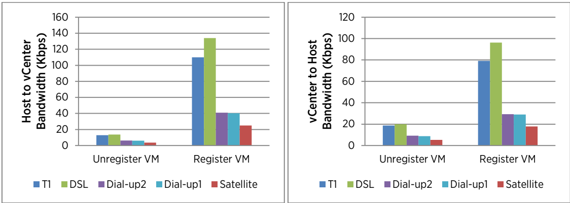
Figure 14. Bandwidth consumption for unregistering and registering a VM. The more bandwidth a network pipe has, the more bandwidth is used for a vCenter task. However, the network pipes are not saturated for all the five representative low-bandwidth cases.
