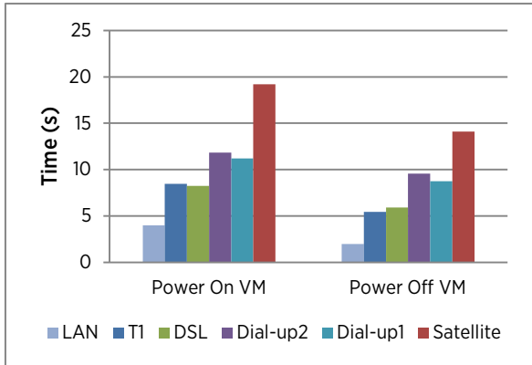
Figure 7. Time consumption for powering on and off a VM. The time consumption increases slowly with network latency.
