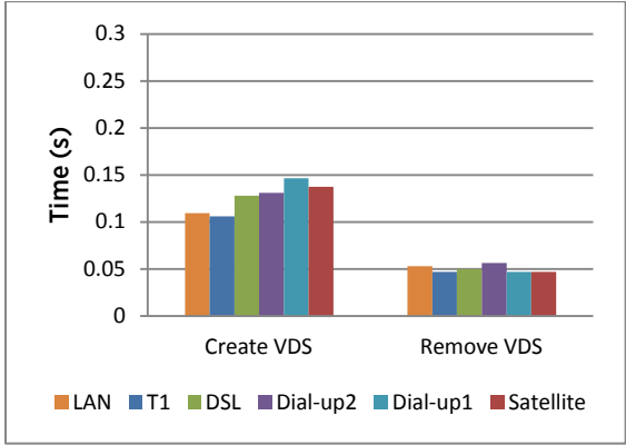
Figure 19. Time consumption for creating and removing a vDS.
