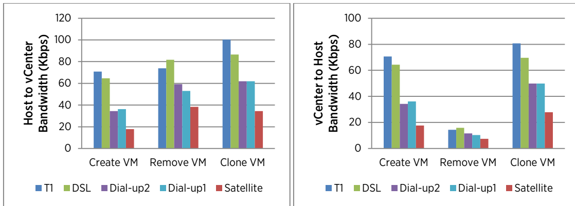
Figure 12. Bandwidth consumption for creating, removing, and cloning a VM. The more bandwidth a network pipe has, the more bandwidth is used for a vCenter task. However, the network pipes are not saturated for all the five representative low-bandwidth cases.
