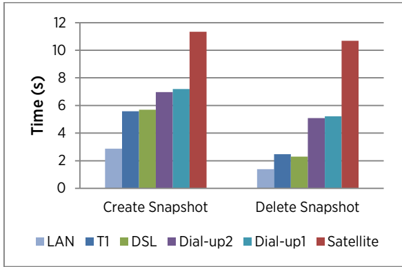
Figure 9. Time consumption for creating and deleting a snapshot. Time consumption increases slowly with network latency.
