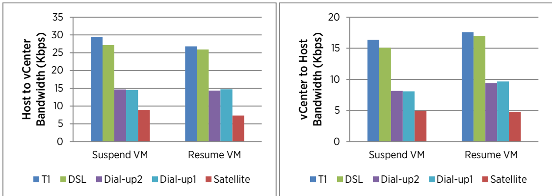
Figure 18. Bandwidth consumption for suspending and resuming a VM. The more bandwidth a network pipe has, the more bandwidth is used for a vCenter task. However, the network pipes are not saturated for all the five representative low-bandwidth cases.
