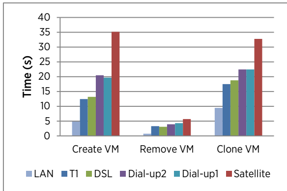
Figure 11. Time consumption for creating, removing, and cloning a VM. The time consumption increases slowly with the network latency.
