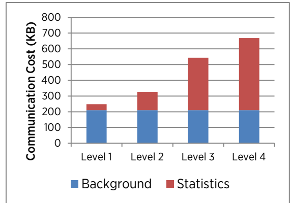
Figure 22. Communication costs of different stats levels for 40 VMs on each host. The blue bar indicates the cost of background traffic and the red bar indicates the cost of statistics traffic
