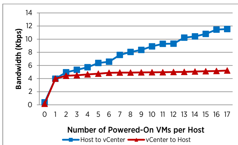
Figure 2. Bandwidth consumption of background traffic. The bandwidth increases linearly with the number of powered-on VMs in each host.
