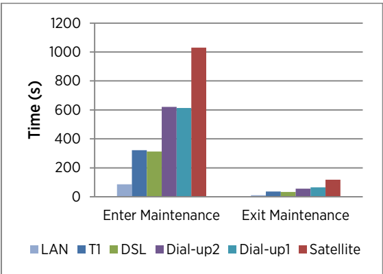
Figure 5. Time consumption for entering and exiting maintenance. The time consumption increases slowly with network latency.
