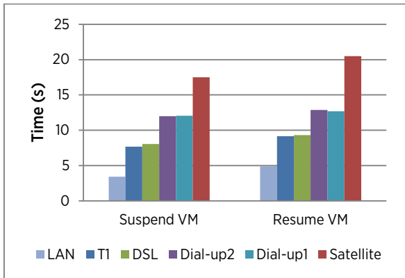
Figure 17. Time consumption for suspending and resuming a VM. Time consumption increases slowly with network latency.
