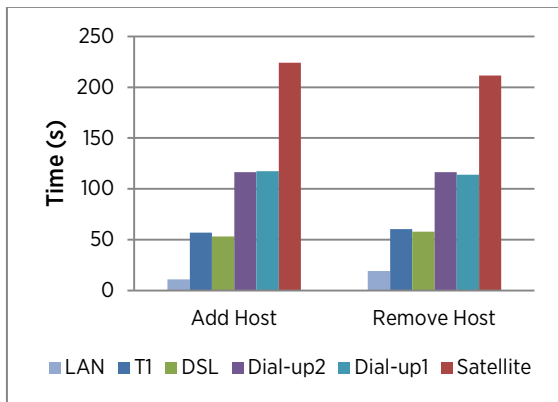
Figure 3. Time consumption for adding and removing a host. The time consumption increases slowly with network latency.
