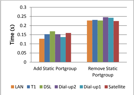
Figure 20. Time consumption for adding and removing a static port group
