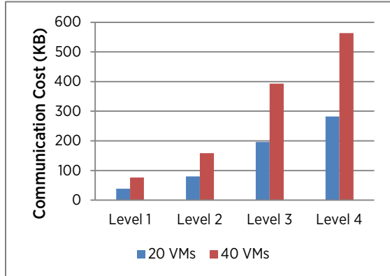
Figure 23. Comparison of overall communication costs for 20 and 40 VMs on each host
