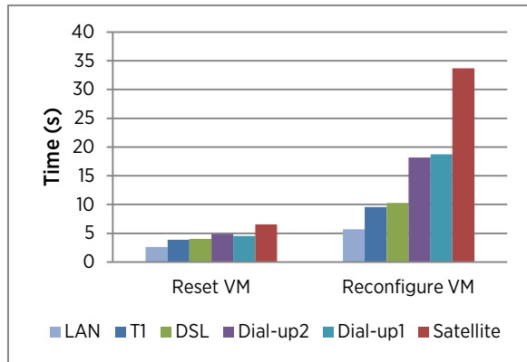
Figure 15. Time consumption for resetting and reconfiguring a VM. The time consumption increases slowly with network latency.
