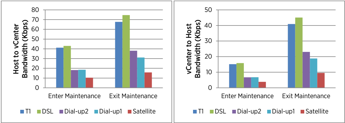
Figure 6. Bandwidth consumption for entering and exiting maintenance mode. The more bandwidth a network pipe has, the more bandwidth is used for a vCenter task. However, the network pipes are not saturated for all the five representative low-bandwidth cases.
