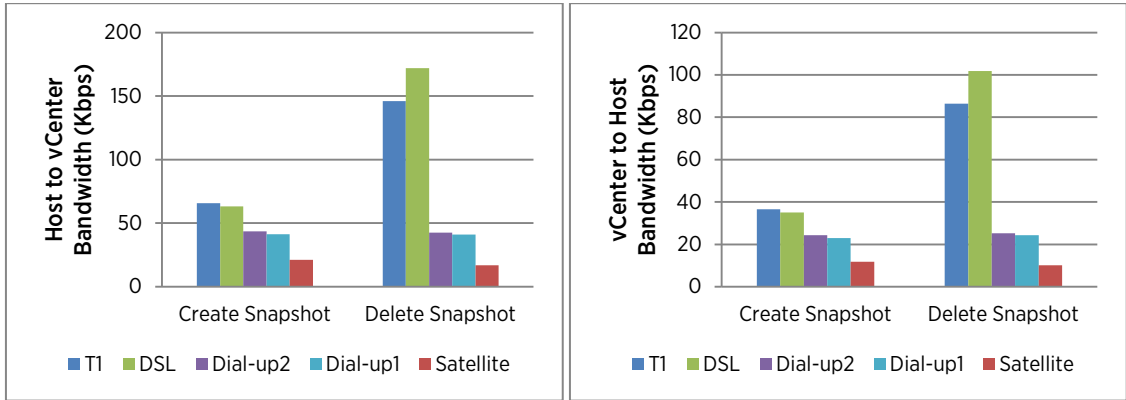
Figure 10. Bandwidth consumption for creating and deleting a snapshot. The more bandwidth a network pipe has, the more bandwidth is used for a vCenter task. However, the network pipes are not saturated for all the five representative low-bandwidth cases.
