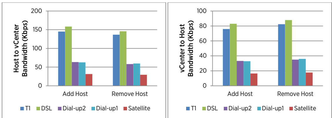
Figure 4. Bandwidth Consumption for adding and removing a host. The more bandwidth a network pipe has, the more bandwidth is used for a vCenter task. However, the network pipes are not saturated for all the five representative low-bandwidth cases.
