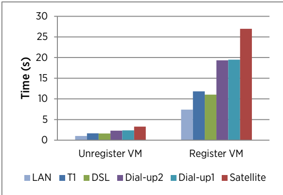
Figure 13. Time consumption for unregistering and registering a VM. The time consumption increases slowly with the network latency.
