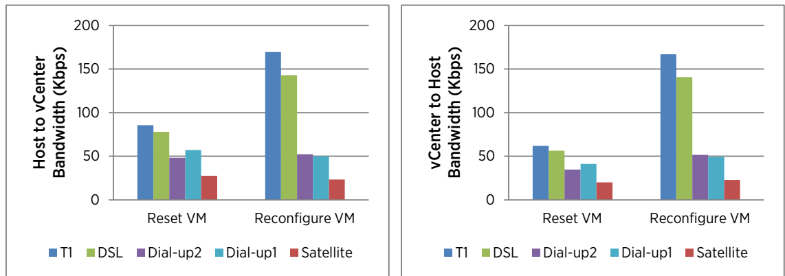
Figure 16. Bandwidth consumption for resetting and reconfiguring a VM. The more bandwidth a network pipe has, the more bandwidth is used for a vCenter task. However, the network pipes are not saturated for all the five representative low-bandwidth cases.
