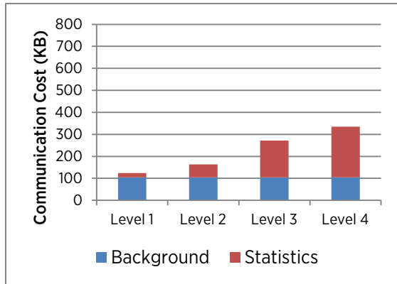
Figure 21. Communication costs of different stats levels for 20 VMs on each host. The blue bar indicates the cost of background traffic and the red bar indicates the cost of statistics traffic.
