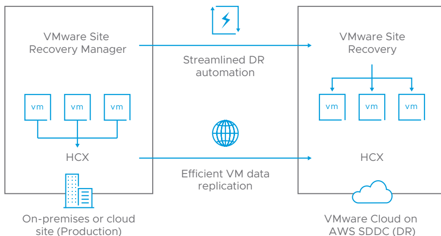
FIGURE 2: Disaster recovery with VCF Operations HCX and VMware Site Recovery Manager.
