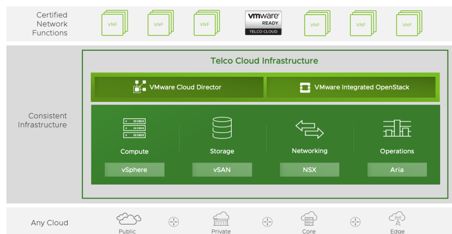
FIGURE 1: The architecture of VMware Telco Cloud Infrastructure, which provides infrastructure to simplify, scale, and protect the operation of multi-vendor network functions.
