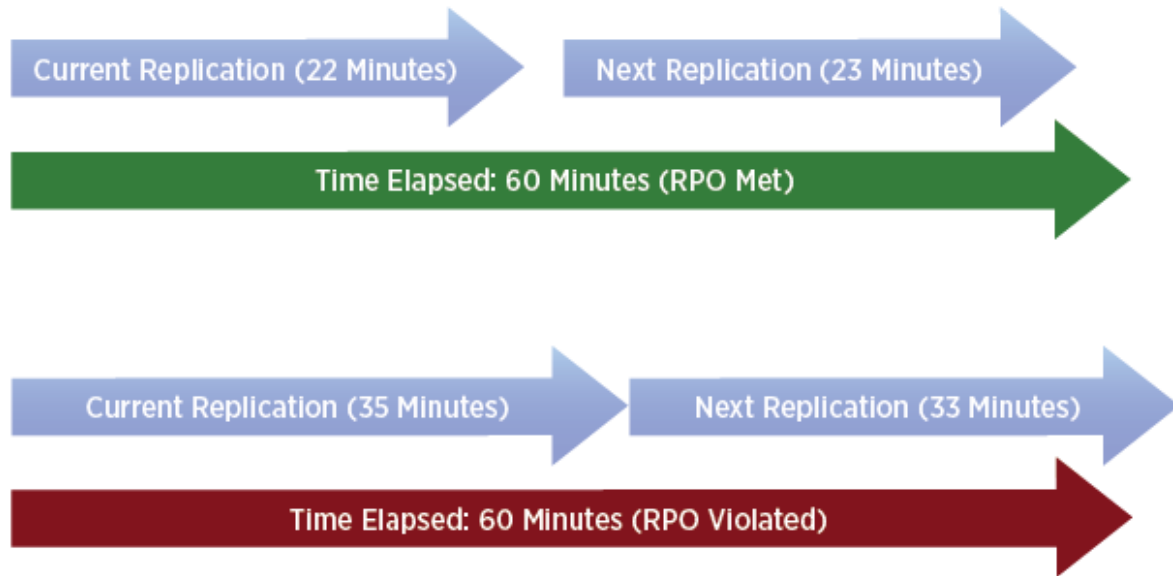
Figure 1. vSphere Replication Schedule Generation
