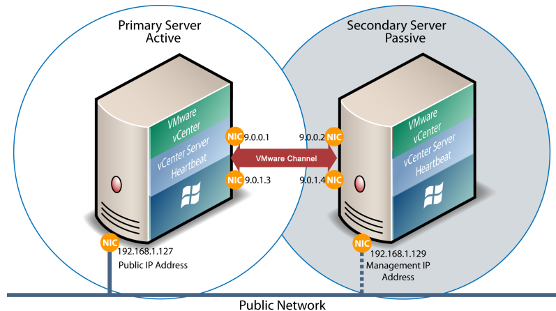
Figure 1- 1. Communications Between Primary and Secondary Servers
