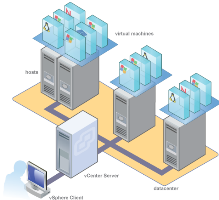
Figure 3. vSphere Components
