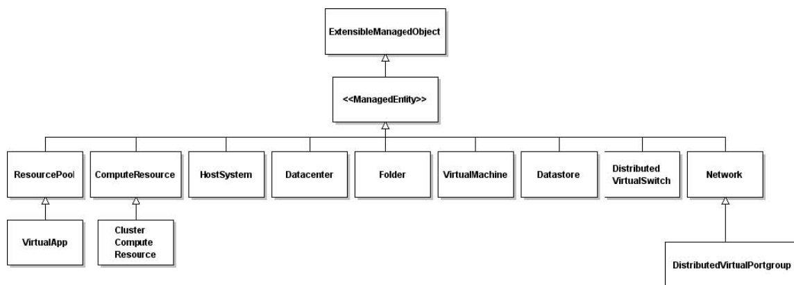
Figure 2-1. ExtensibleManagedEntity Hierarchy
